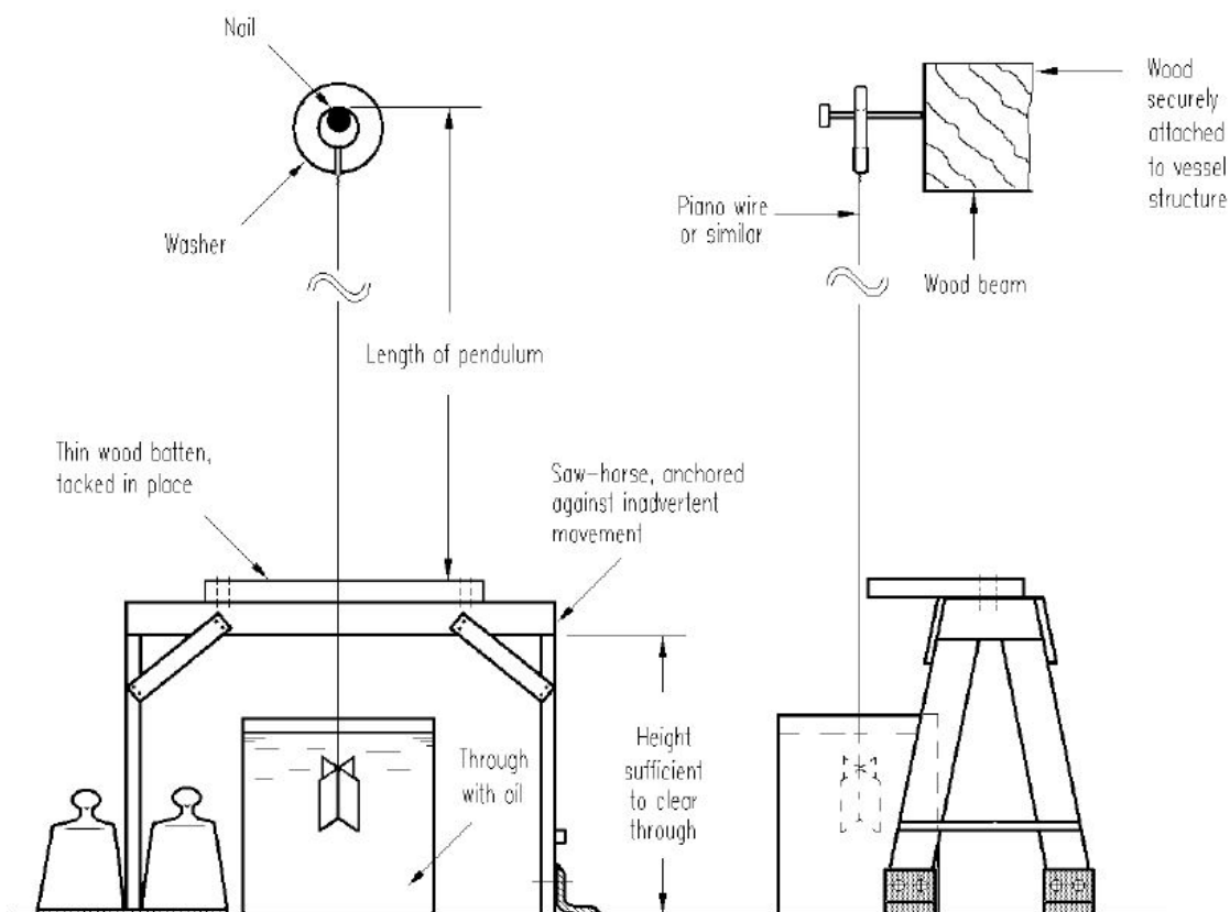
Fig. 1 Recommended set-up of pendulums
