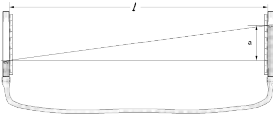
Fig. 2 Reading of U-tube
